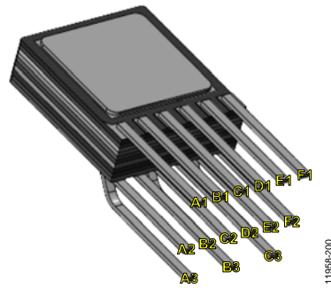
Figure 4. Pin Configuration (3D View)
