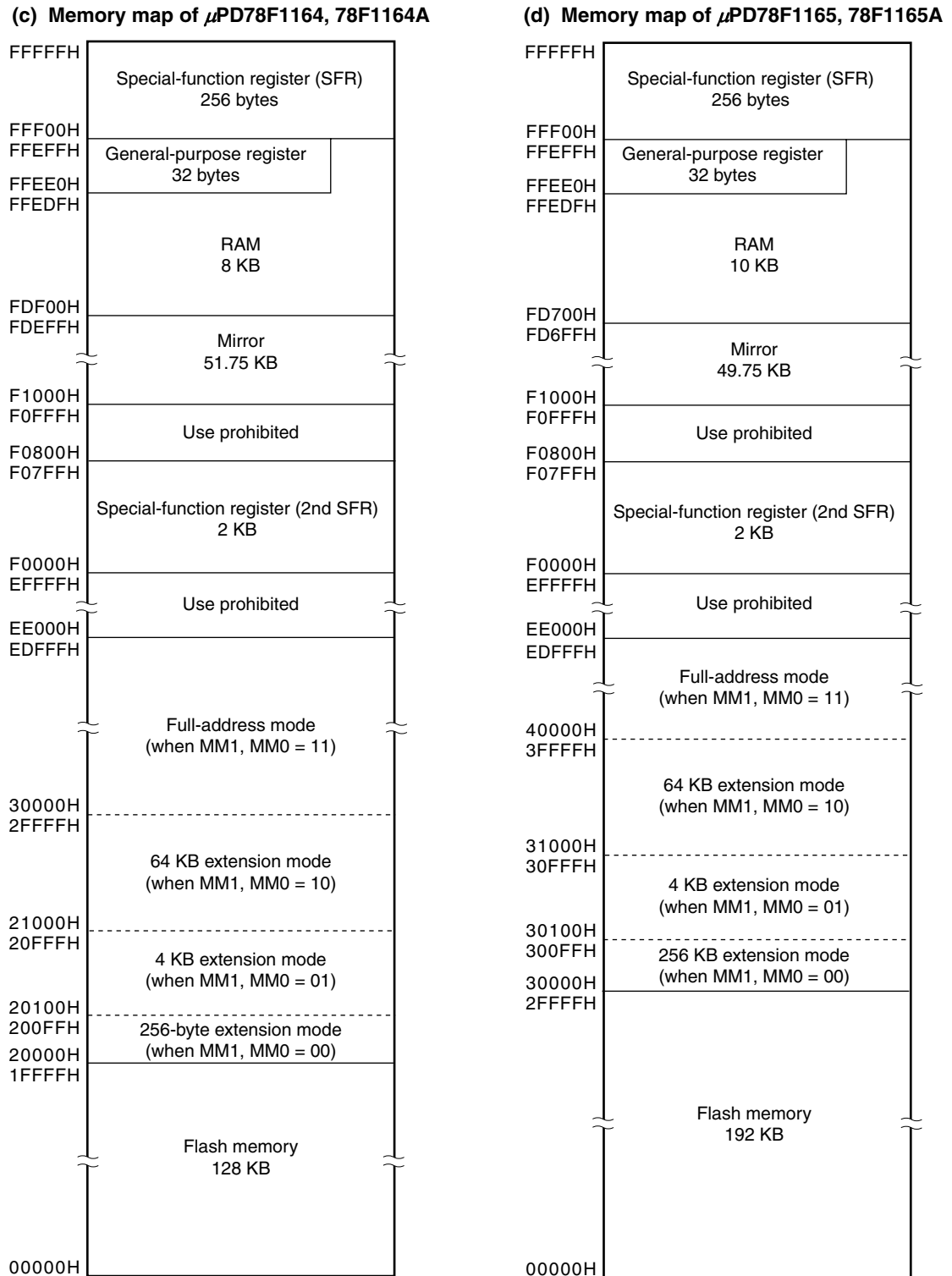
Figure 5-1. Memory Map When Using External Bus Interface Function (2/4)
