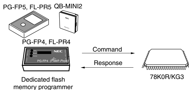
Figure 25-10. Communication Commands
