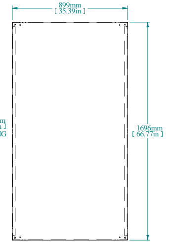
INNER PANEL
