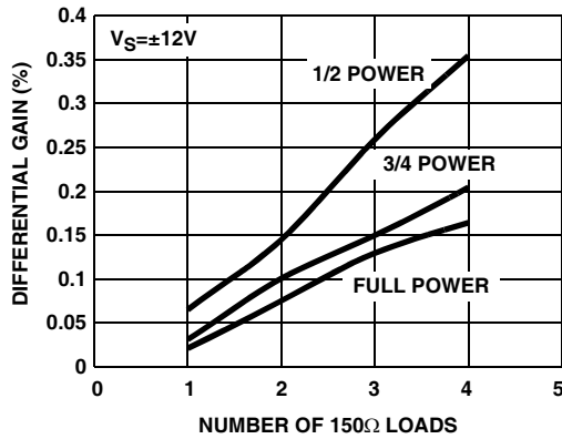
FIGURE 37. DIFFERENTIAL GAIN
