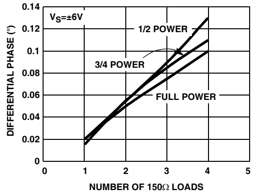
FIGURE 38. DIFFERENTIAL PHASE
