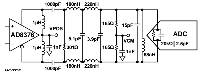
Figure 42. Differential Input Configuration Using the AD8376
