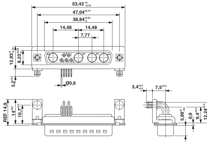
Dimensioned drawing
