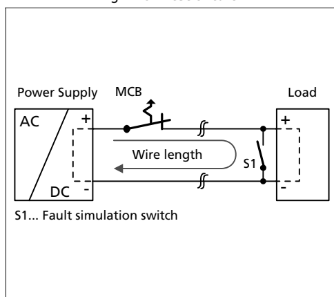
Fig. 24-9 Test circuit
