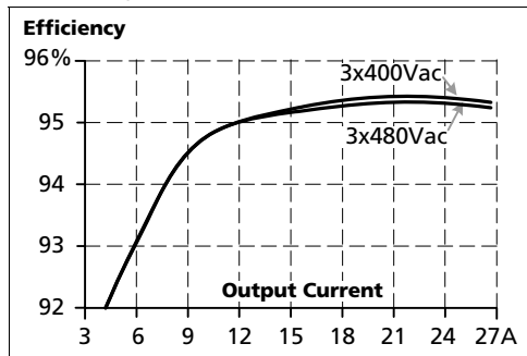
Fig. 11-1 Efficiency vs. output current at 36V, typ.
