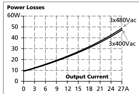
Fig. 11-2 Losses vs. output current at 36V, typ.
