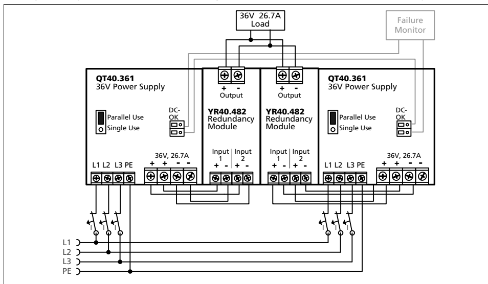
Fig. 23-1 Typical 1+1 Redundant configuration for 26.7A with a dual redundancy module
