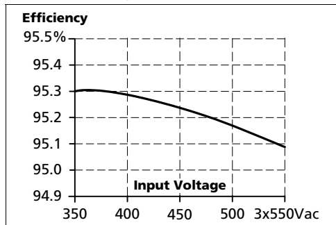
Fig. 11-3 Efficiency vs. input voltage at 36V, 26.7A, typ.
