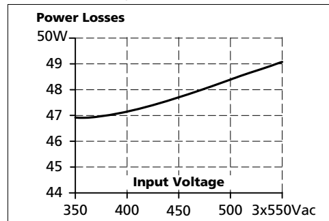
Fig. 11-4 Losses vs. input voltage at 36V, 26.7A, typ.
