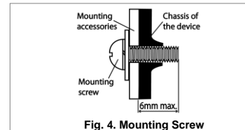
Fig. 4. Mounting Screw
