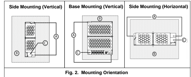
Fig. 2. Mounting Orientation
