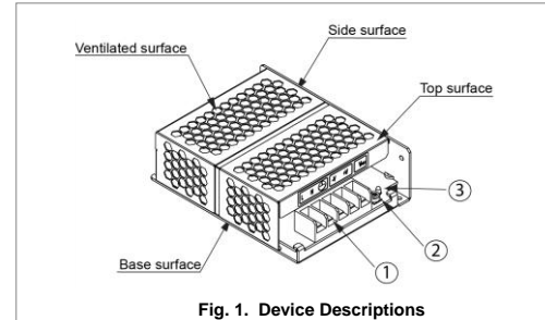
Fig. 1. Device Descriptions
